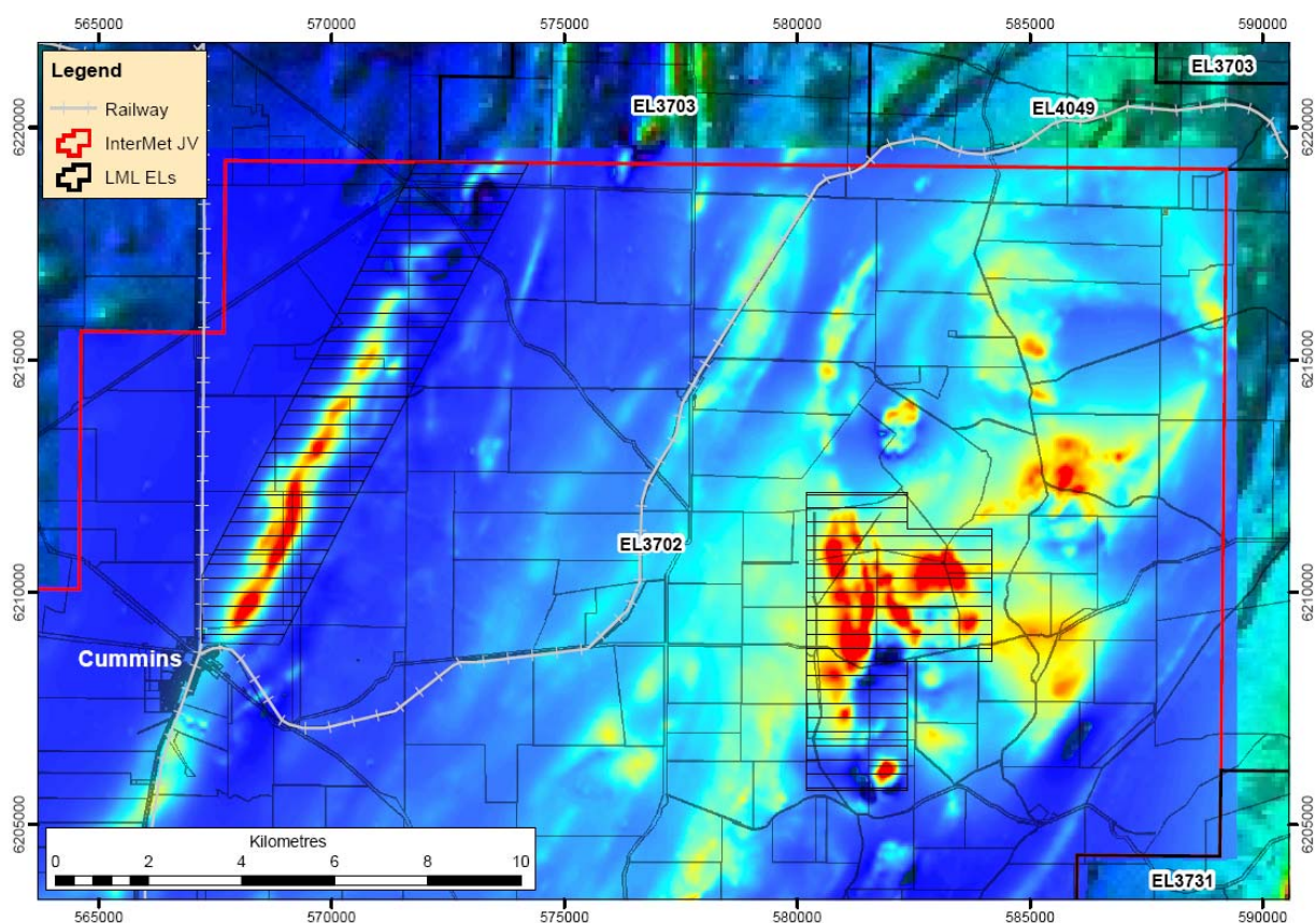
Figure 1: Location of detailed gravity grids on EL 3702
