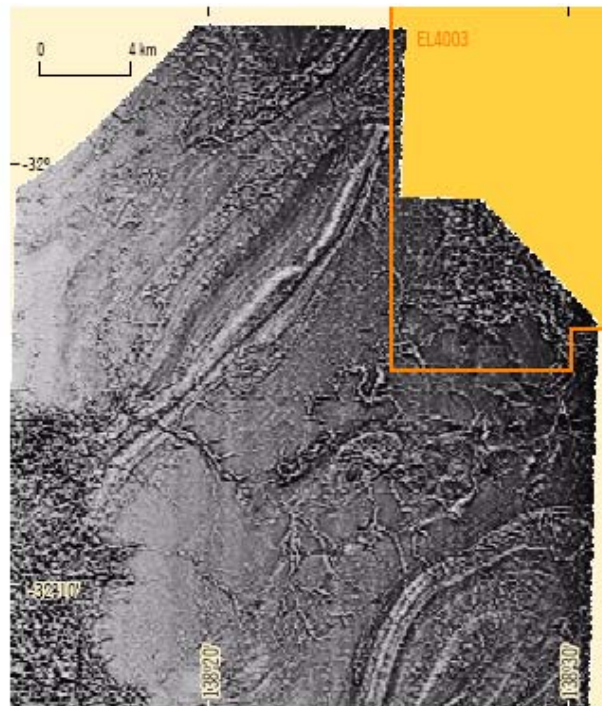
Figure 2: New magnetic data (1VD image)
